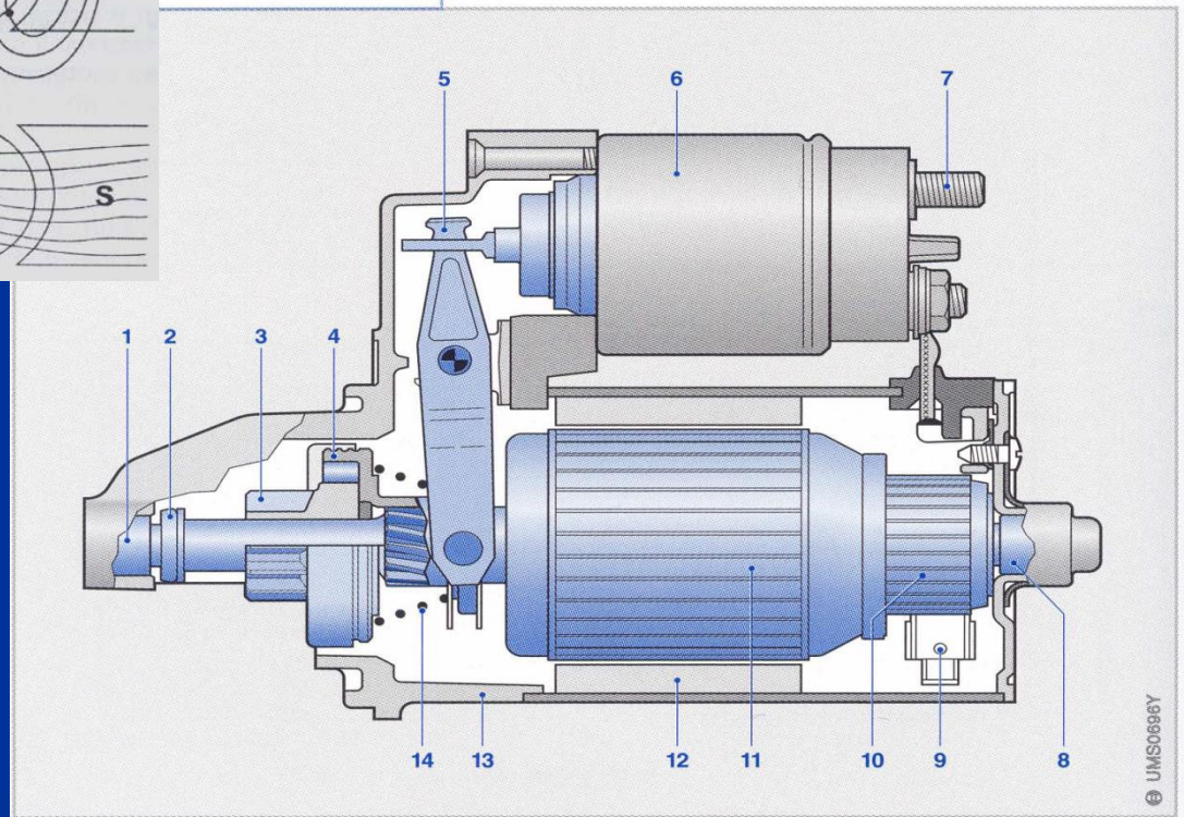
78 direct-drive starter motor
